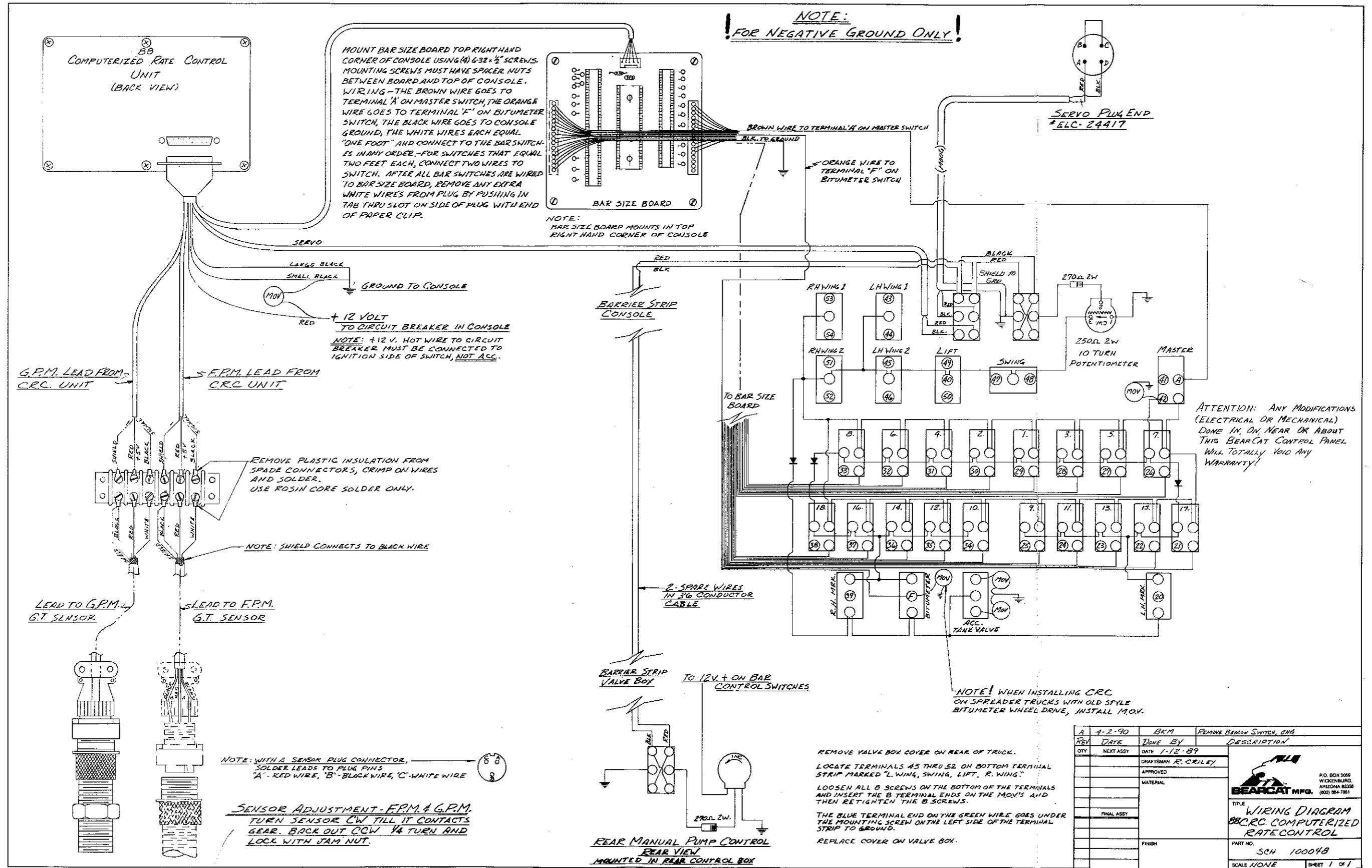
(FIGURE 6.24) CRC WIRING DIAGRAM
