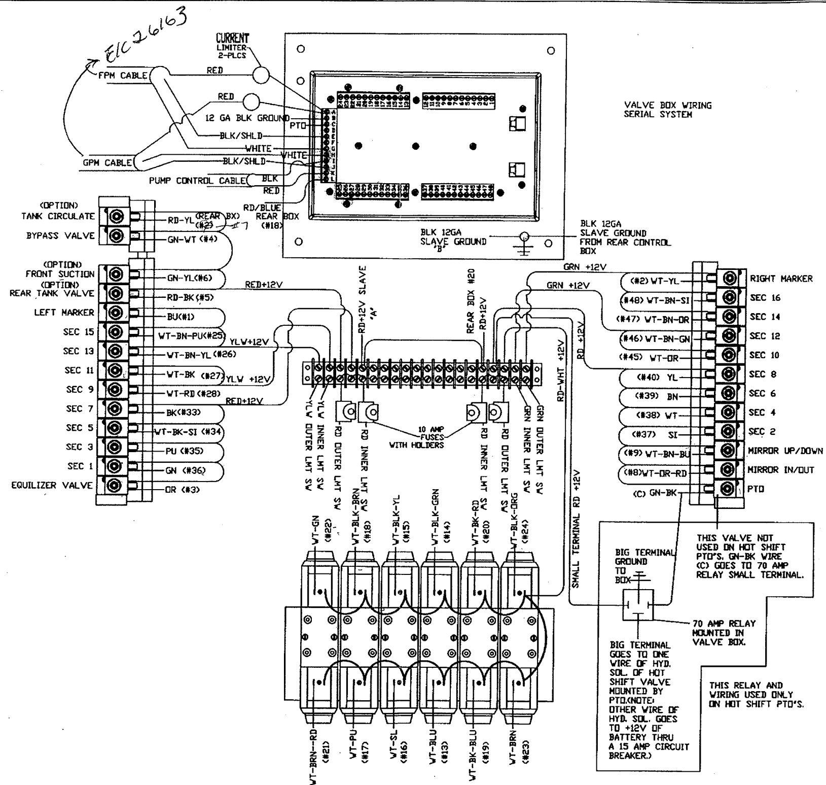
Figure 9-2. Schematic Valve Box
